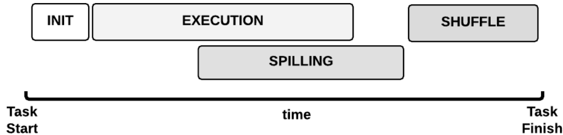
Fig. Map Task execution timeline:
